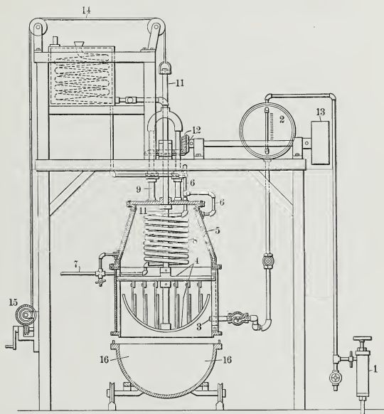
FIG. 34.—Priest's Condenser. 1. Naphtha pump. 2. Tank. 4. Stirrer. 11. Elevating shaft for same. 12, 13. Driving mechanism. 5. Cold-water jacket. 8. Cold-water coil. 15. Worm-gear for raising and lowering the condenser.
